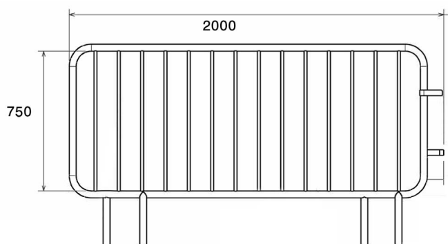
4 coins arrondis
